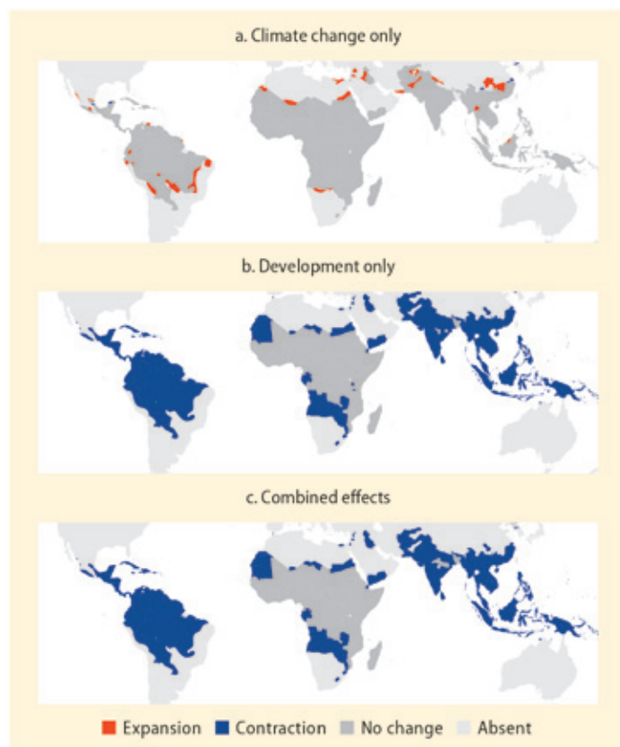
MAP 4.2 By 2050, socioeconomic development should reduce malaria incidence, even with climate change
